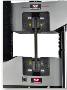
G7 - Open Front with Hydraulic Actuation
